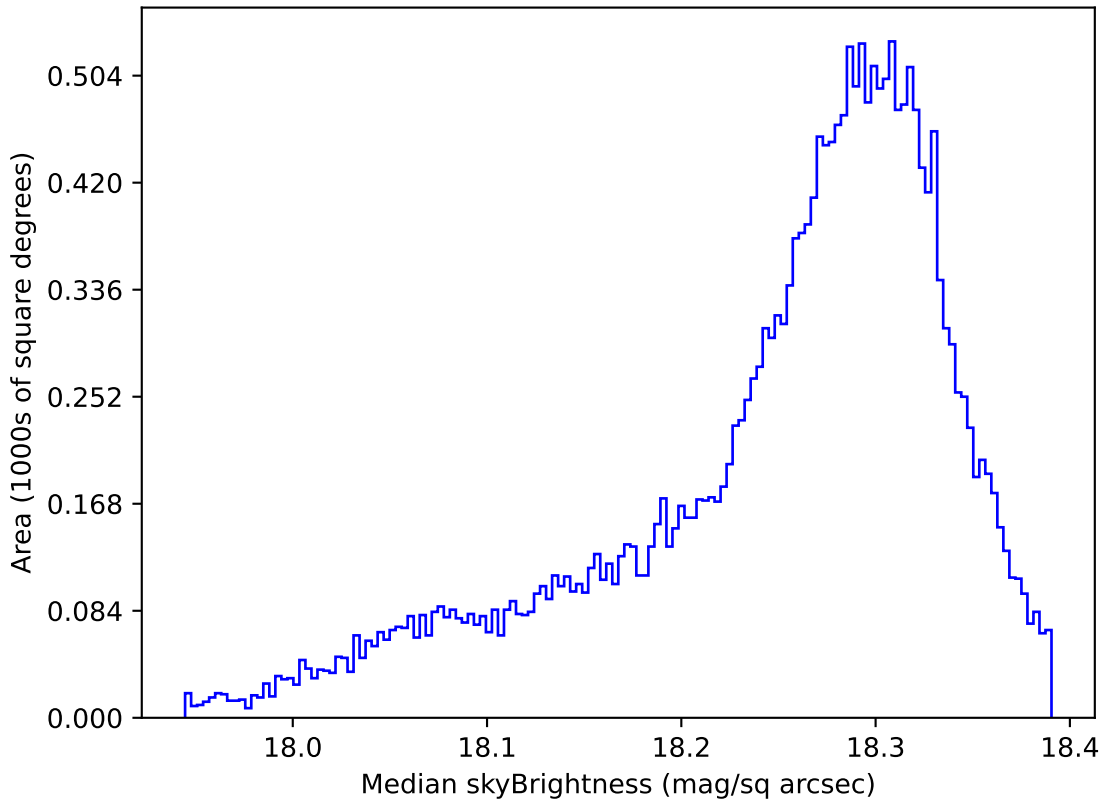
weather_cloudso2v3.4_10yrs All sky y band: Median skyBrightness
