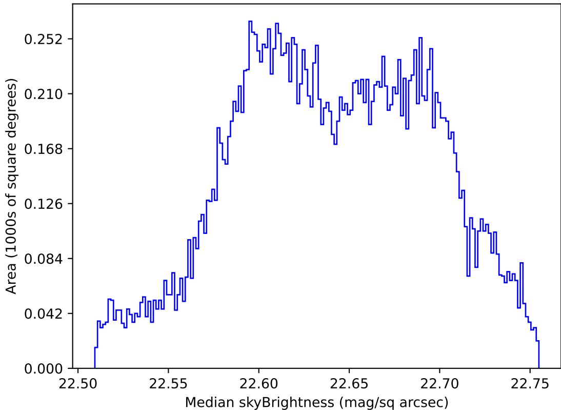
weather_cloudso2v3.4_10yrs All sky u band: Median skyBrightness
