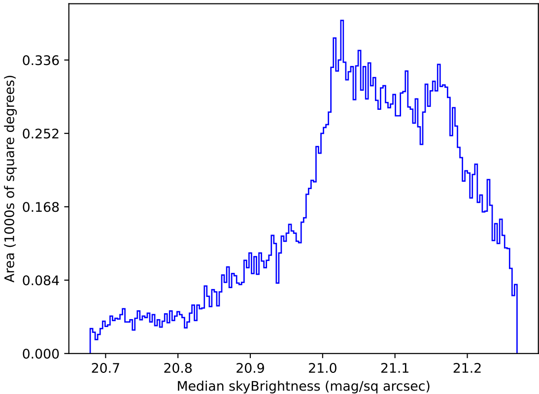
weather_cloudso2v3.4_10yrs All sky r band: Median skyBrightness
