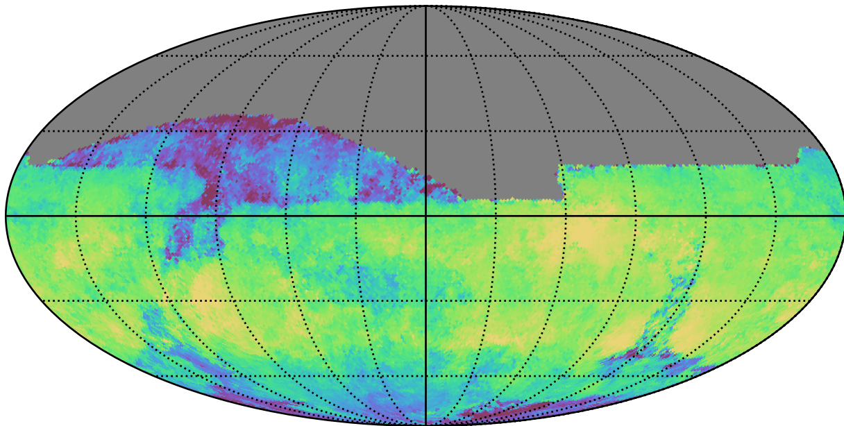
weather_cloudso2v3.4_10yrs All sky i band: Median skyBrightness
