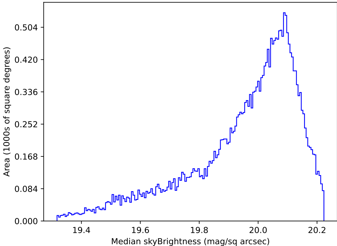
weather_cloudso2v3.4_10yrs All sky i band: Median skyBrightness
