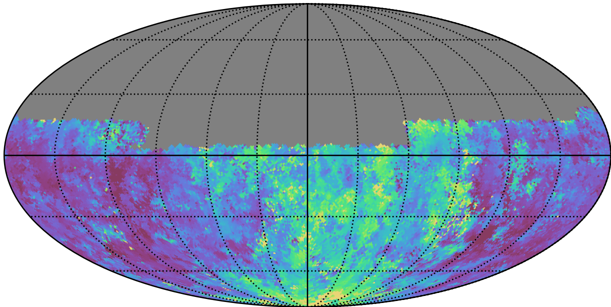
weather_cloudso2v3.4_10yrs Yr 1 u band: Median seeingGeom
