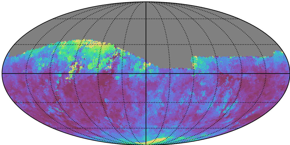
weather_cloudso2v3.4_10yrs Yr 1 r band: Median seeingGeom
