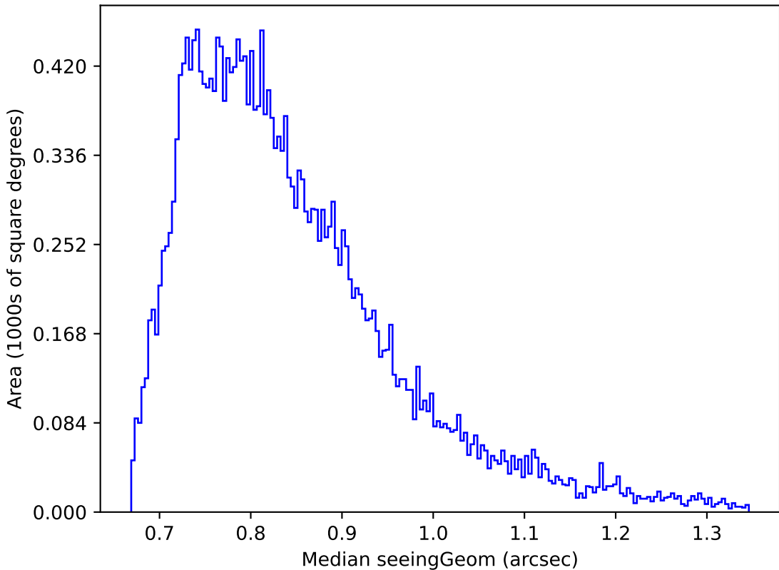
weather_cloudso2v3.4_10yrs Yr 1 r band: Median seeingGeom
