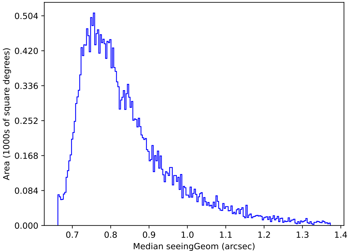
weather_cloudso2v3.4_10yrs Yr 1 i band: Median seeingGeom
