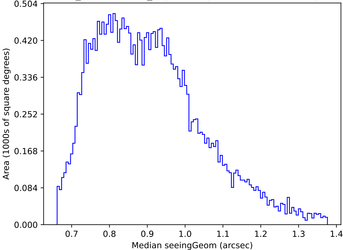
weather_cloudso2v3.4_10yrs Yr 1 g band: Median seeingGeom
