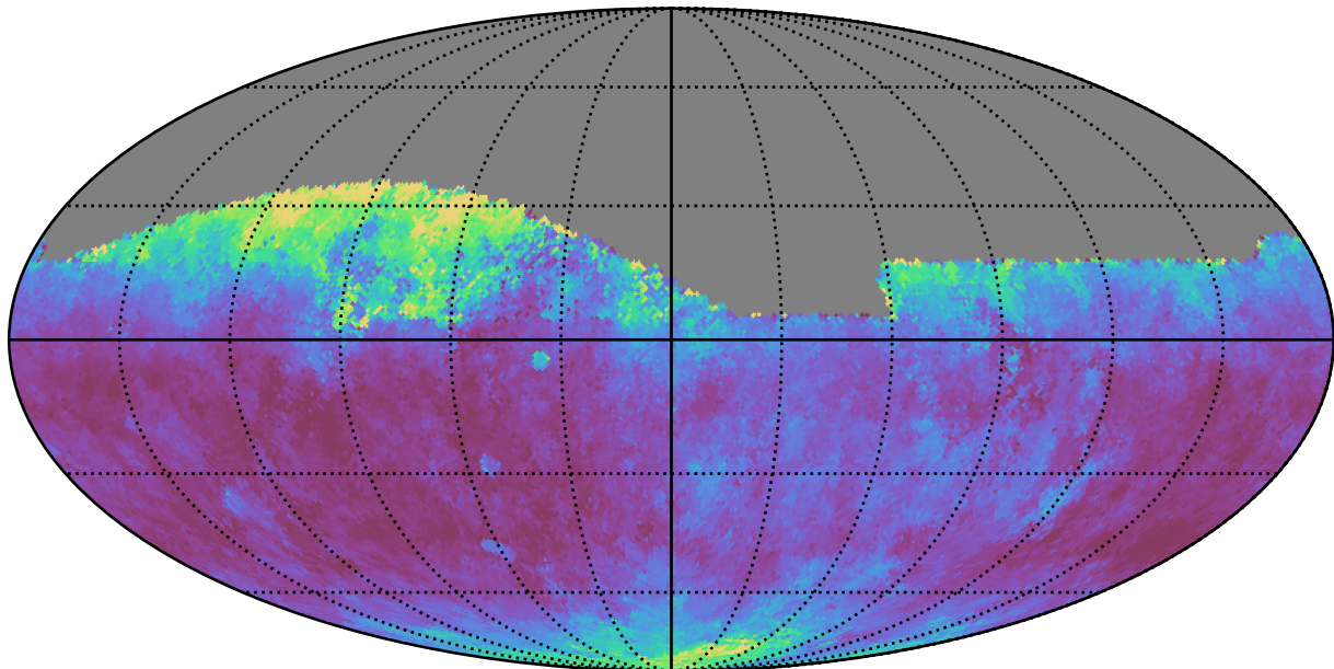
weather_cloudso2v3.4_10yrs Yr 1 all bands: Median seeingGeom
