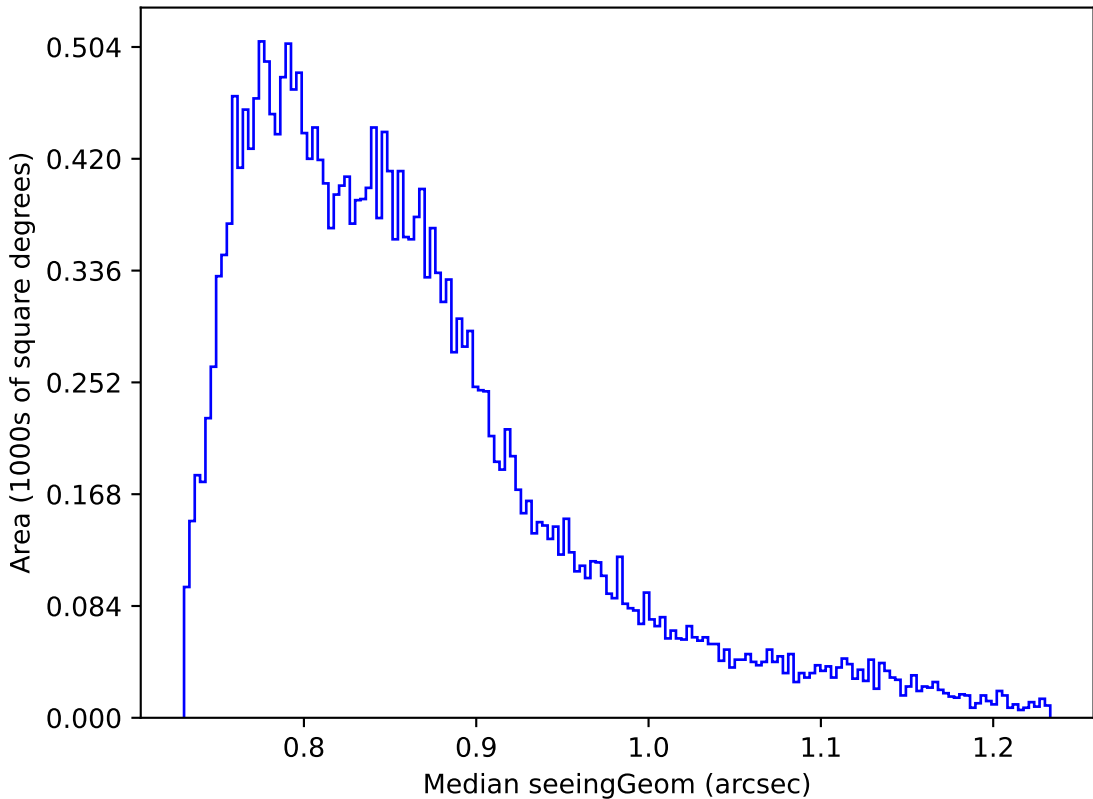
weather_cloudso2v3.4_10yrs Yr 1 all bands: Median seeingGeom
