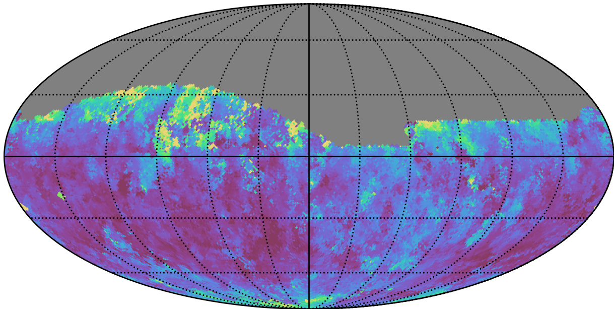
weather_cloudso2v3.4_10yrs Yr 1 z band: Median seeingEff
