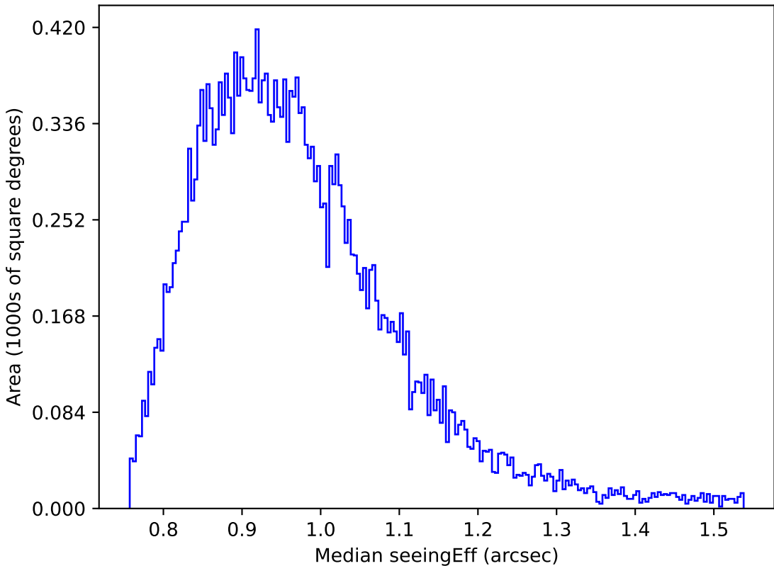
weather_cloudso2v3.4_10yrs Yr 1 z band: Median seeingEff
