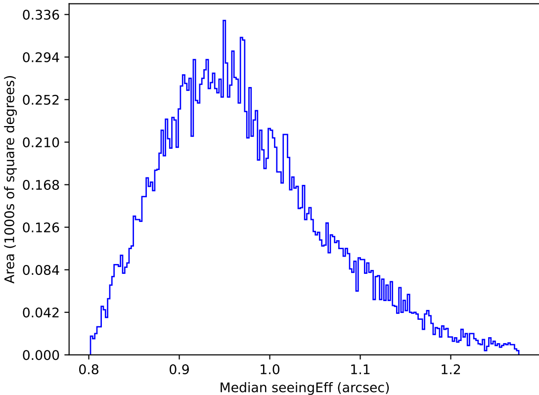
weather_cloudso2v3.4_10yrs Yr 1 y band: Median seeingEff
