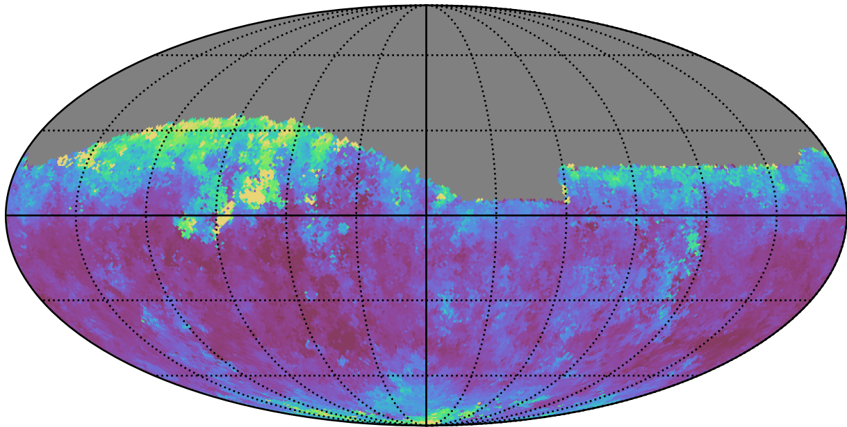
weather_cloudso2v3.4_10yrs Yr 1 i band: Median seeingEff
