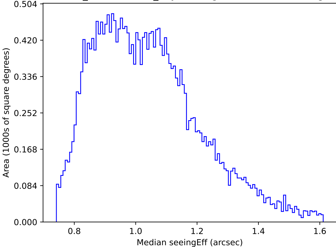
weather_cloudso2v3.4_10yrs Yr 1 g band: Median seeingEff
