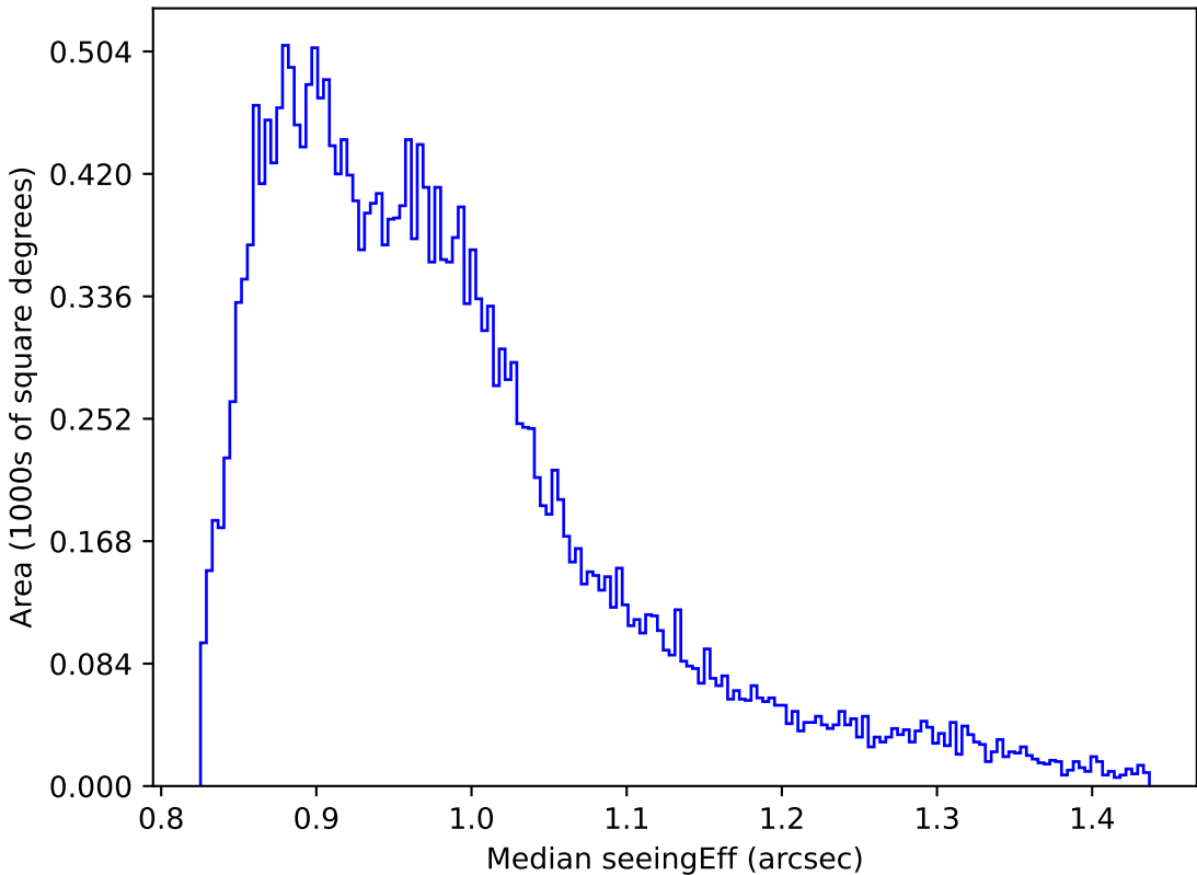
weather_cloudso2v3.4_10yrs Yr 1 all bands: Median seeingEff
