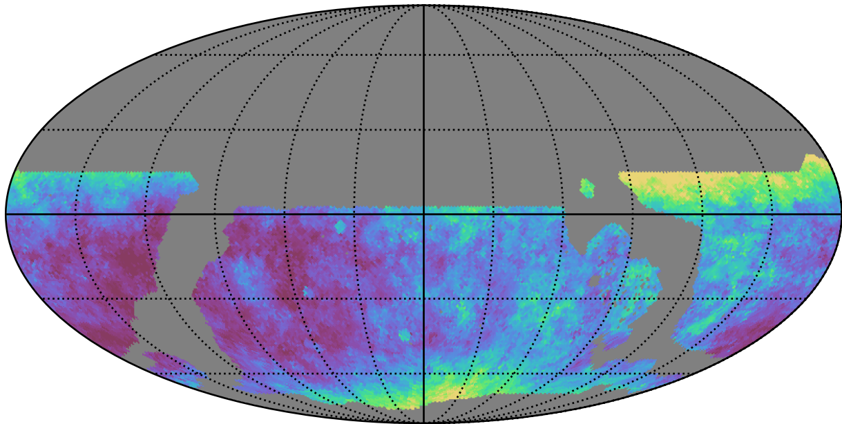
weather_cloudso2v3.4_10yrs WFD y band: Median seeingEff
