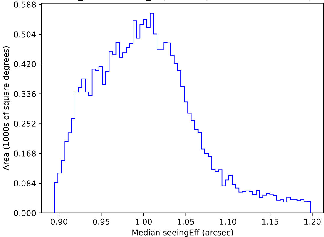
weather_cloudso2v3.4_10yrs WFD y band: Median seeingEff
