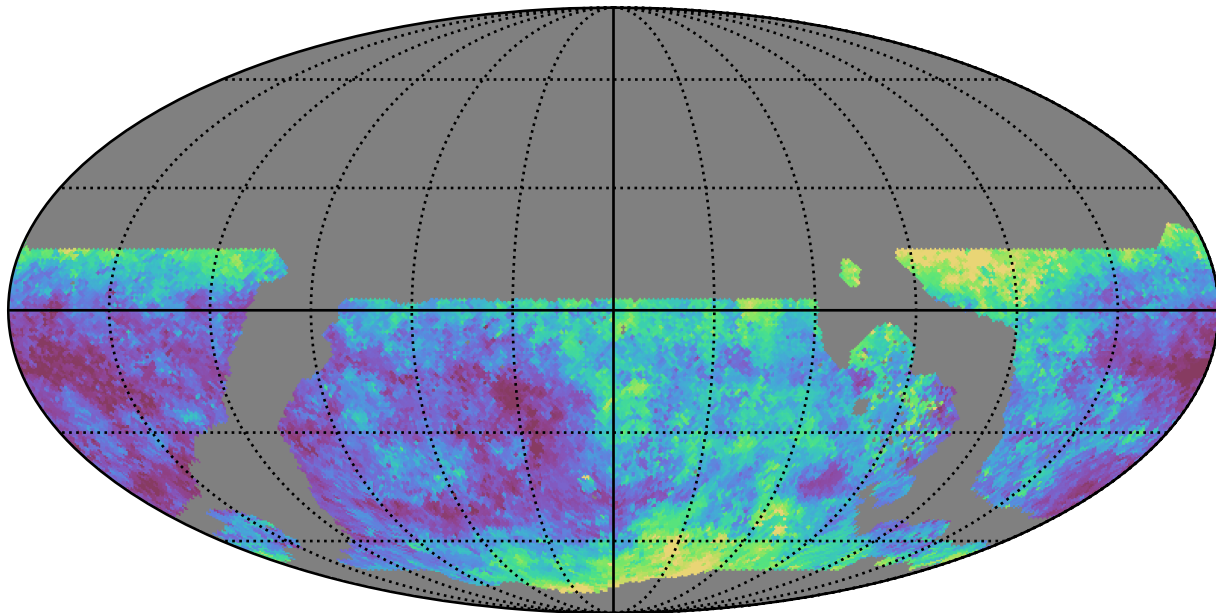
weather_cloudso2v3.4_10yrs WFD u band: Median seeingEff
