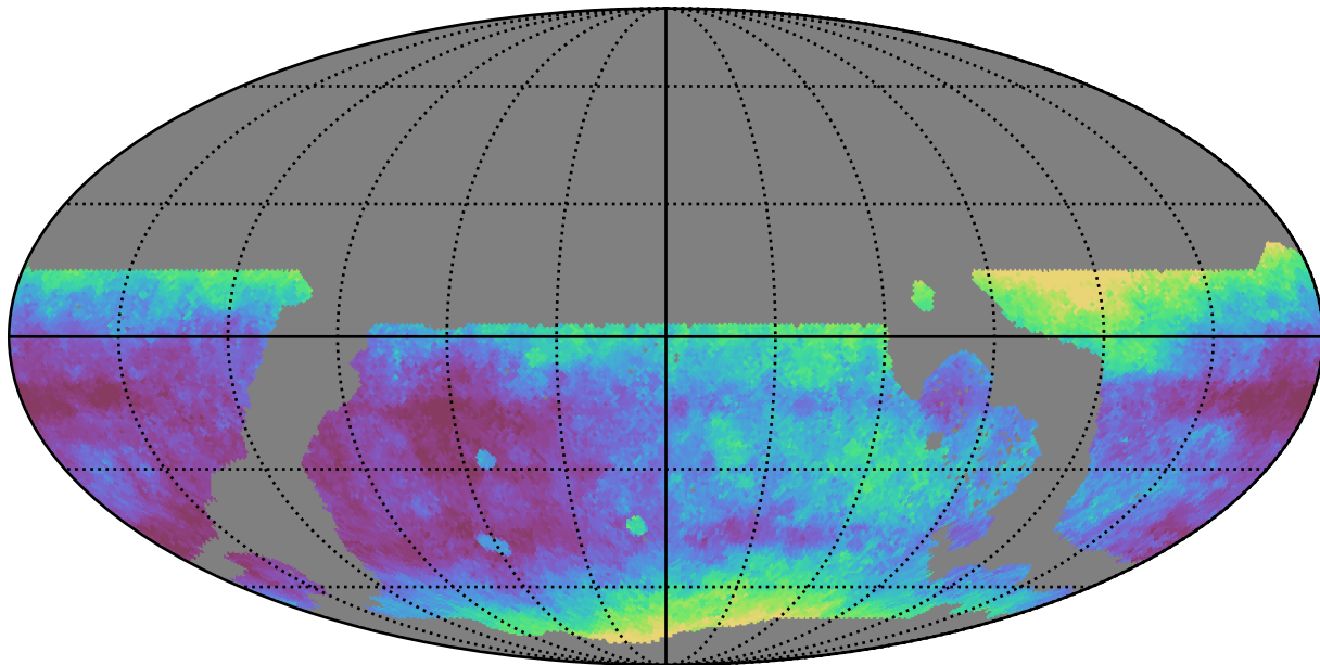
weather_cloudso2v3.4_10yrs WFD r band: Median seeingEff
