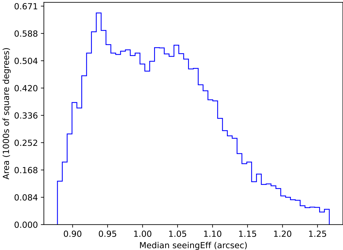
weather_cloudso2v3.4_10yrs WFD r band: Median seeingEff
