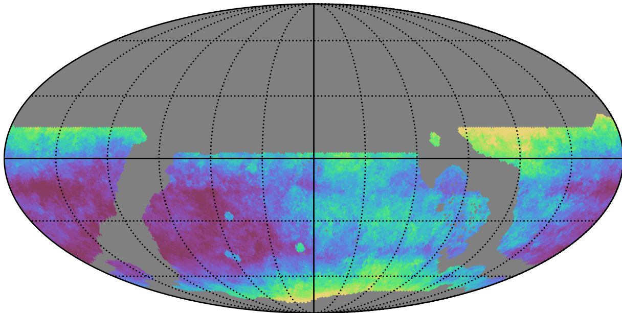
weather_cloudso2v3.4_10yrs WFD i band: Median seeingEff
