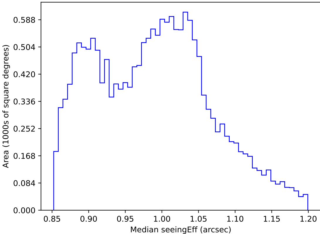
weather_cloudso2v3.4_10yrs WFD i band: Median seeingEff
