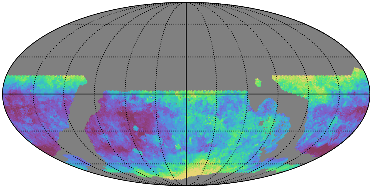
weather_cloudso2v3.4_10yrs WFD g band: Median seeingEff
