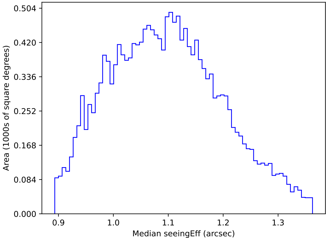
weather_cloudso2v3.4_10yrs WFD g band: Median seeingEff
