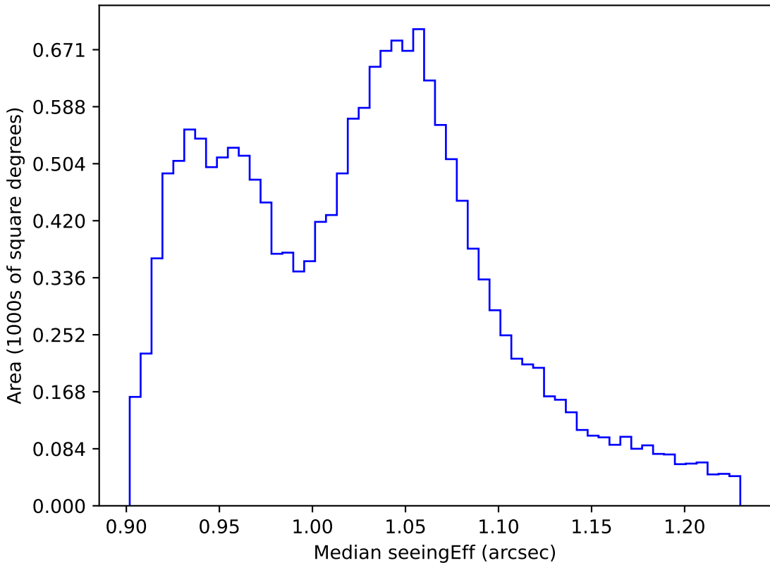
weather_cloudso2v3.4_10yrs WFD all bands: Median seeingEff
