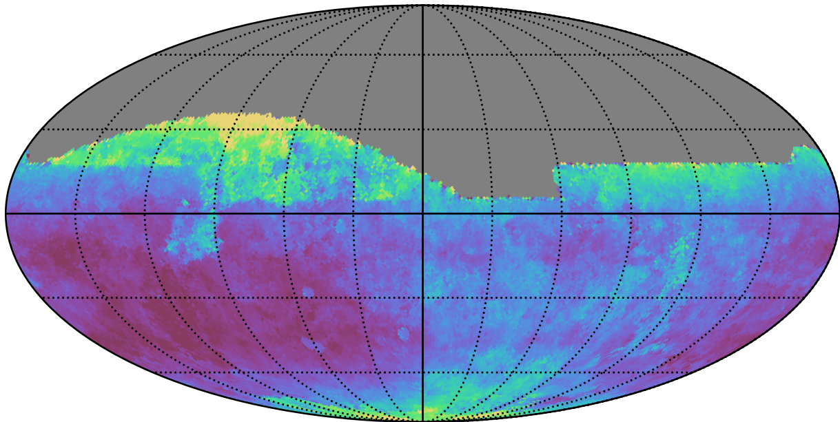
weather_cloudso2v3.4_10yrs All sky z band: Median seeingEff
