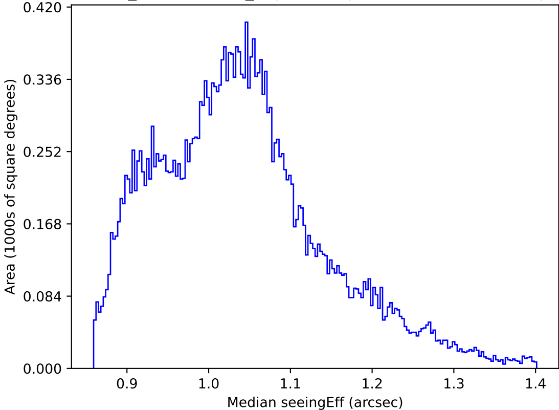
weather_cloudso2v3.4_10yrs All sky z band: Median seeingEff
