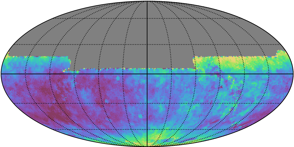
weather_cloudso2v3.4_10yrs All sky y band: Median seeingEff
