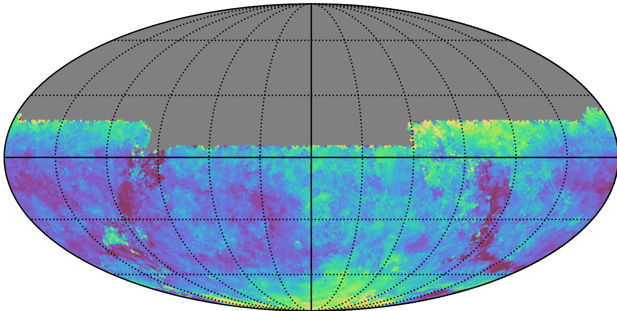
weather_cloudso2v3.4_10yrs All sky u band: Median seeingEff
