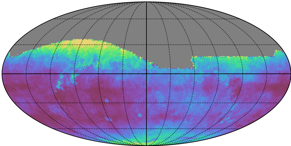
weather_cloudso2v3.4_10yrs All sky r band: Median seeingEff
