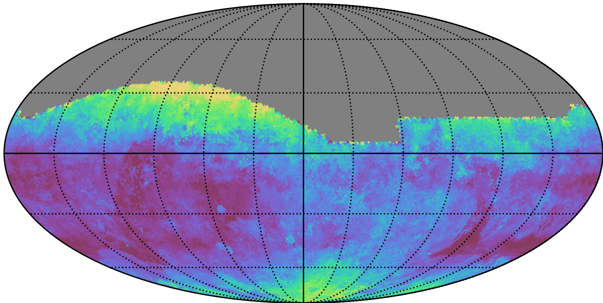
weather_cloudso2v3.4_10yrs All sky g band: Median seeingEff
