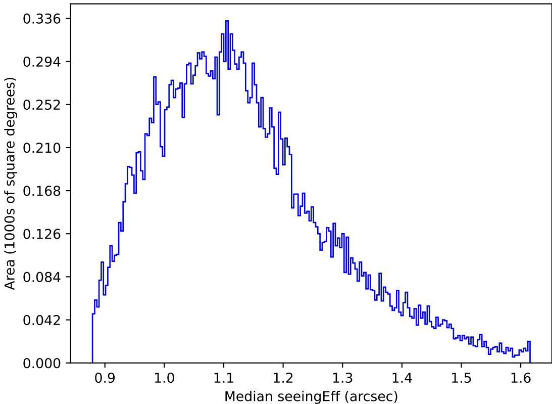
weather_cloudso2v3.4_10yrs All sky g band: Median seeingEff
