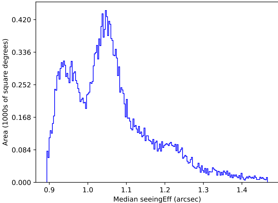
weather_cloudso2v3.4_10yrs All sky all bands: Median seeingEff
