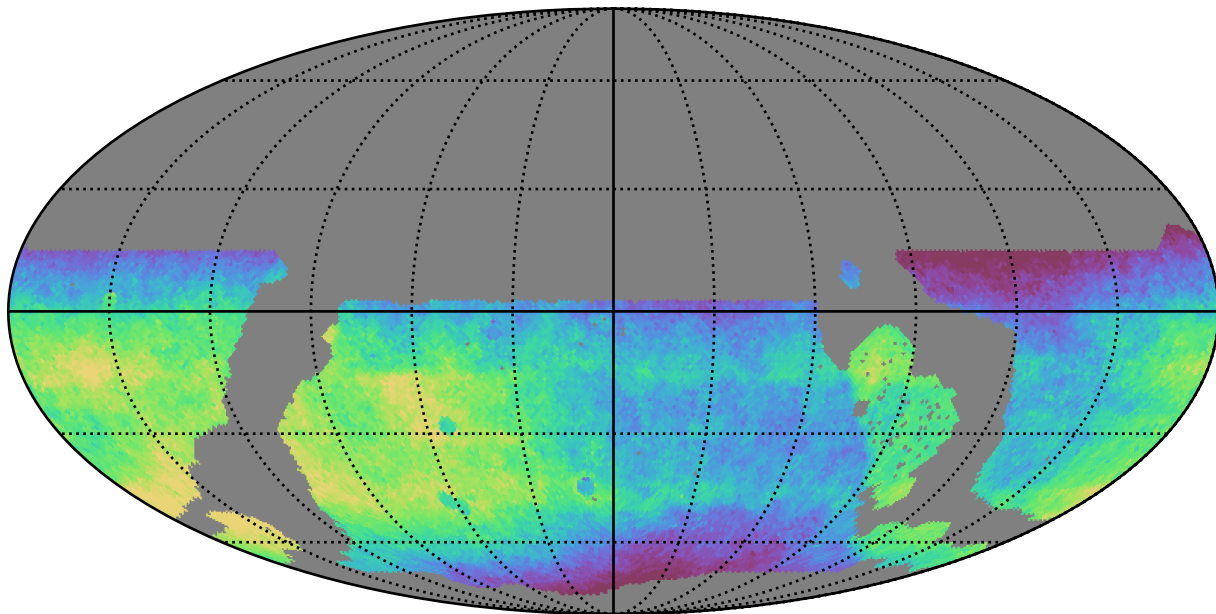
weather_cloudso2v3.4_10yrs WFD all bands: Median saturation_mag
