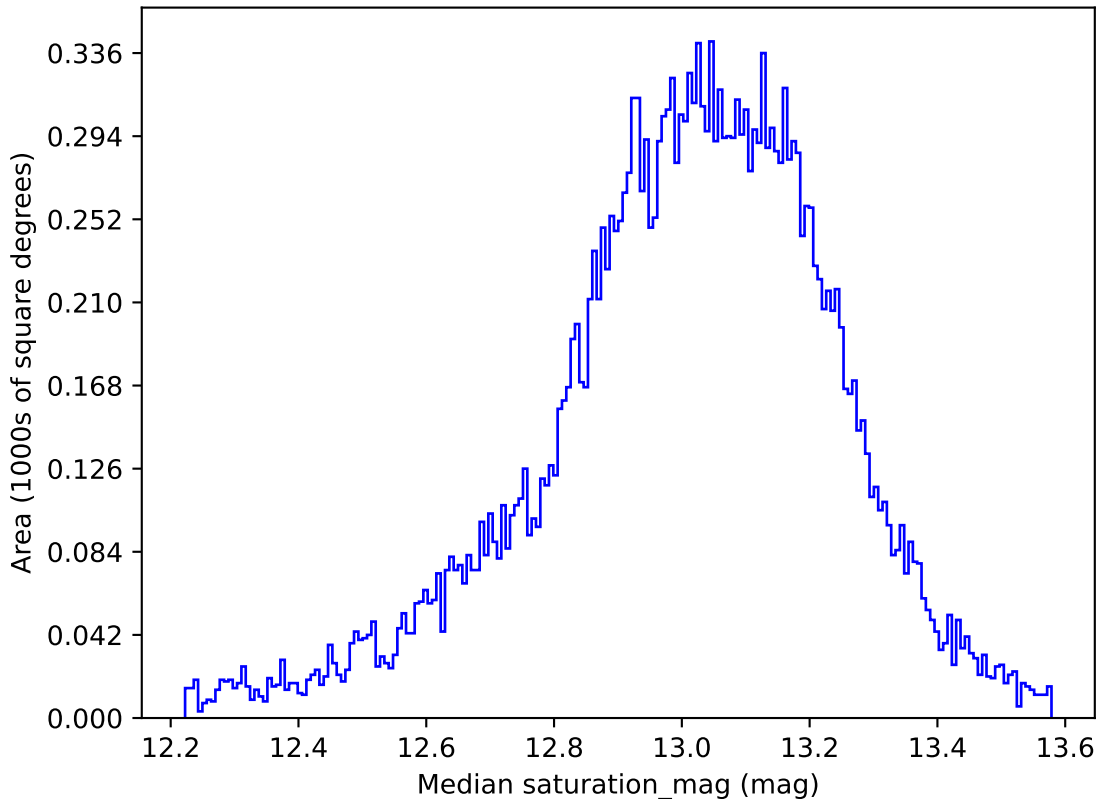
weather_cloudso2v3.4_10yrs All sky u band: Median saturation_mag
