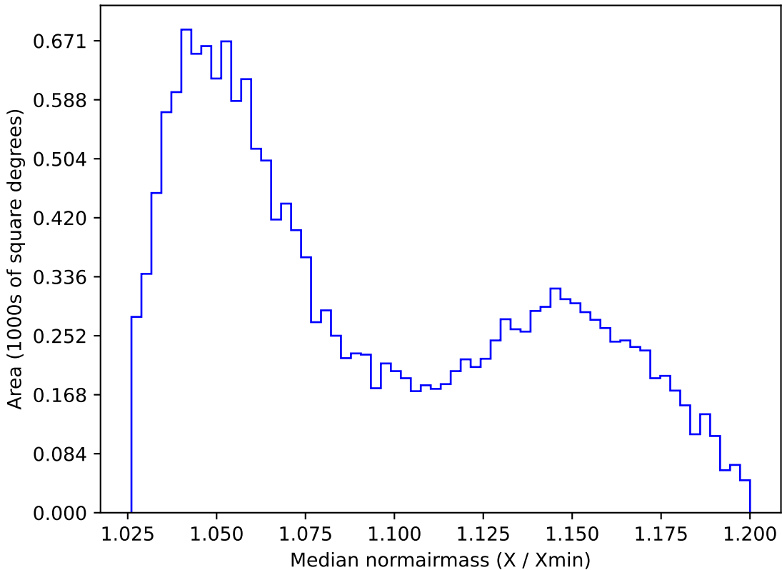
weather_cloudso2v3.4_10yrs WFD z band: Median normairmass
