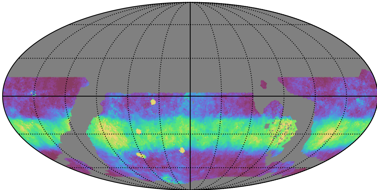
weather_cloudso2v3.4_10yrs WFD y band: Median normairmass
