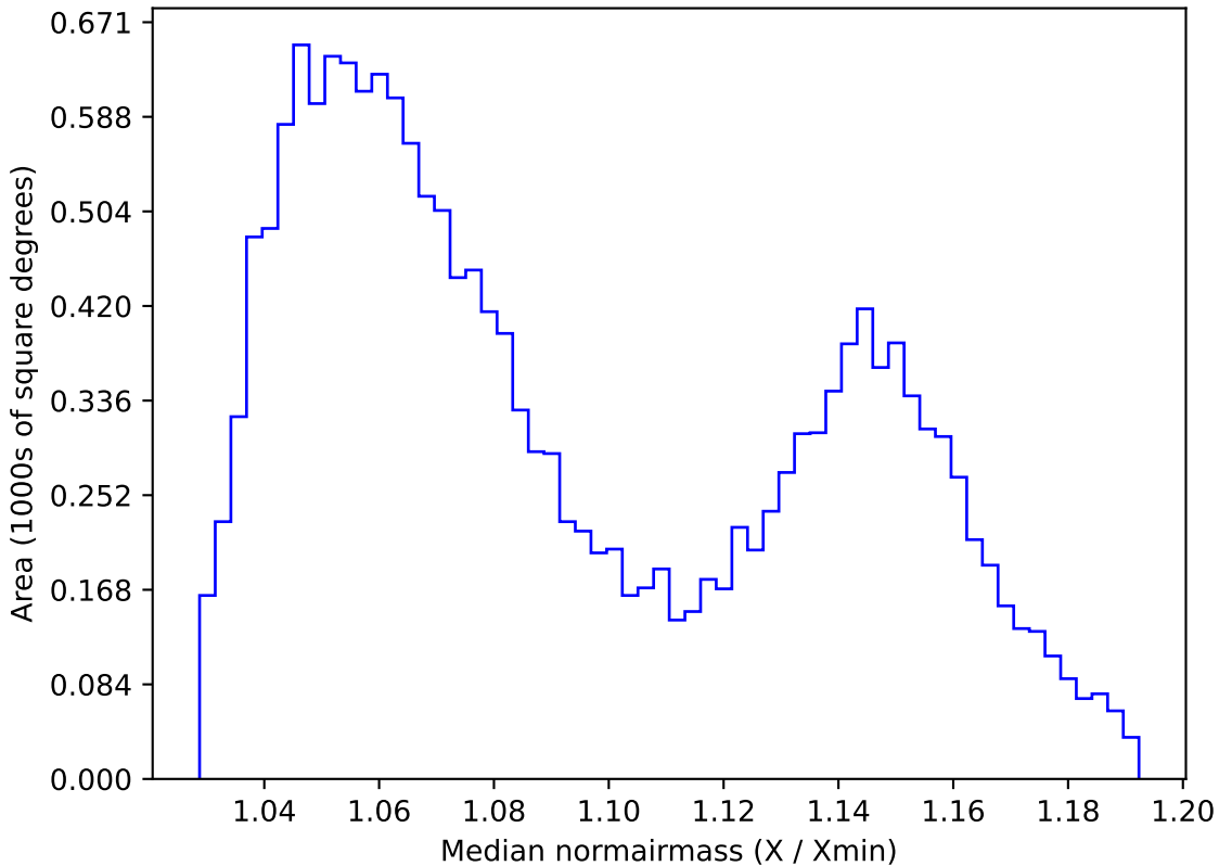
weather_cloudso2v3.4_10yrs WFD y band: Median normairmass
