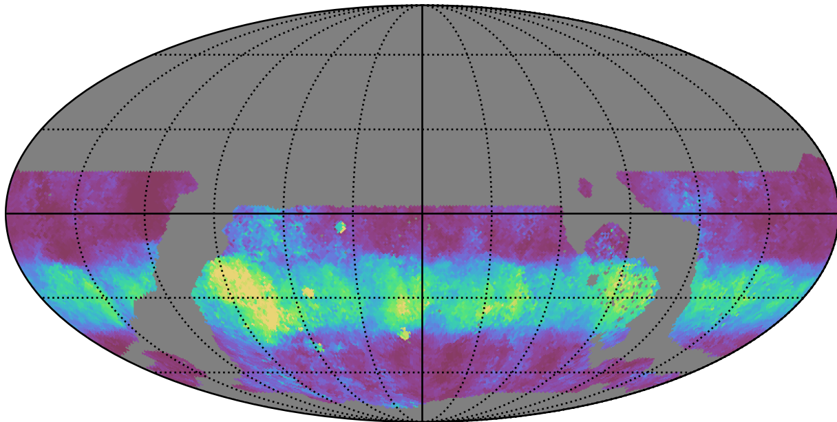
weather_cloudso2v3.4_10yrs WFD u band: Median normairmass
