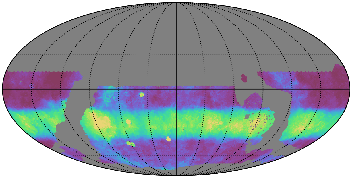
weather_cloudso2v3.4_10yrs WFD r band: Median normairmass
