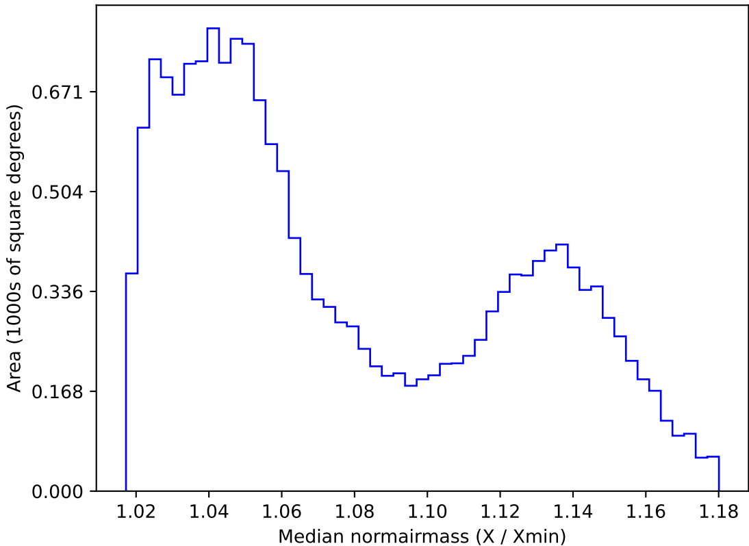
weather_cloudso2v3.4_10yrs WFD r band: Median normairmass
