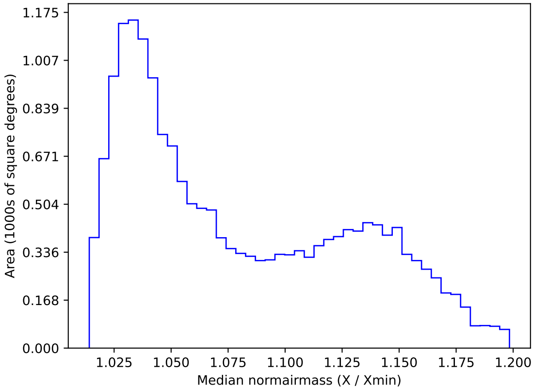
weather_cloudso2v3.4_10yrs WFD g band: Median normairmass
