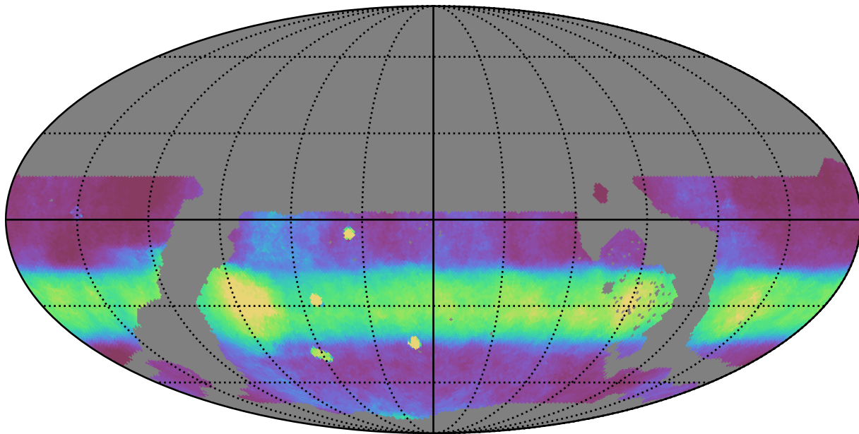
weather_cloudso2v3.4_10yrs WFD all bands: Median normairmass
