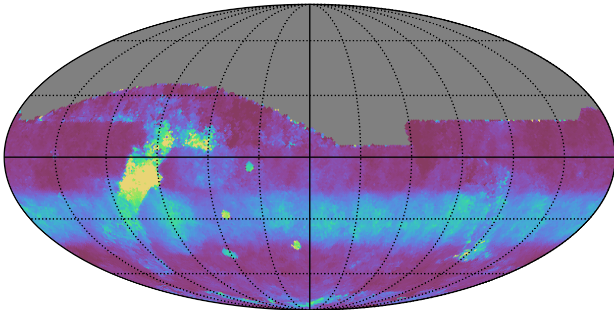
weather_cloudso2v3.4_10yrs All sky z band: Median normairmass
