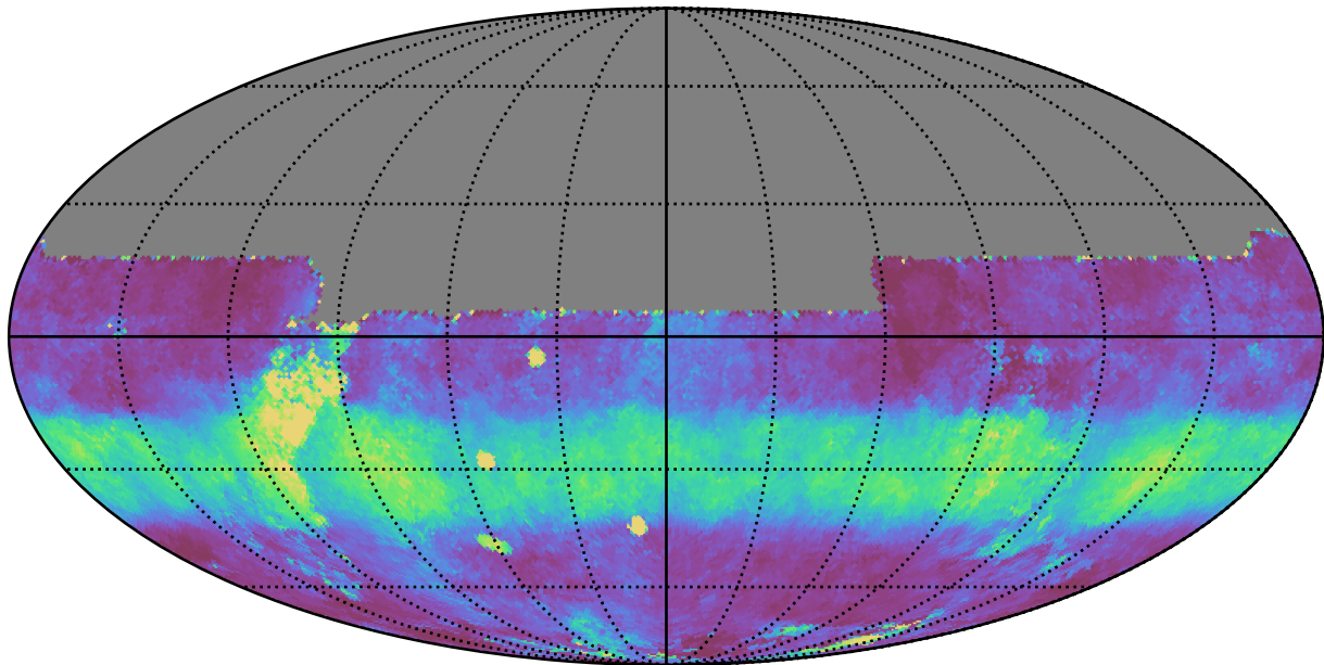
weather_cloudso2v3.4_10yrs All sky y band: Median normairmass
