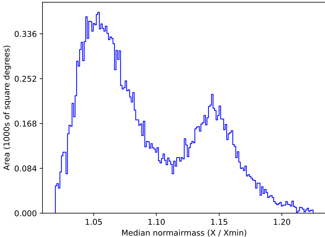
weather_cloudso2v3.4_10yrs All sky y band: Median normairmass
