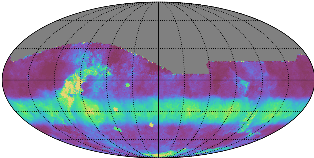
weather_cloudso2v3.4_10yrs All sky r band: Median normairmass
